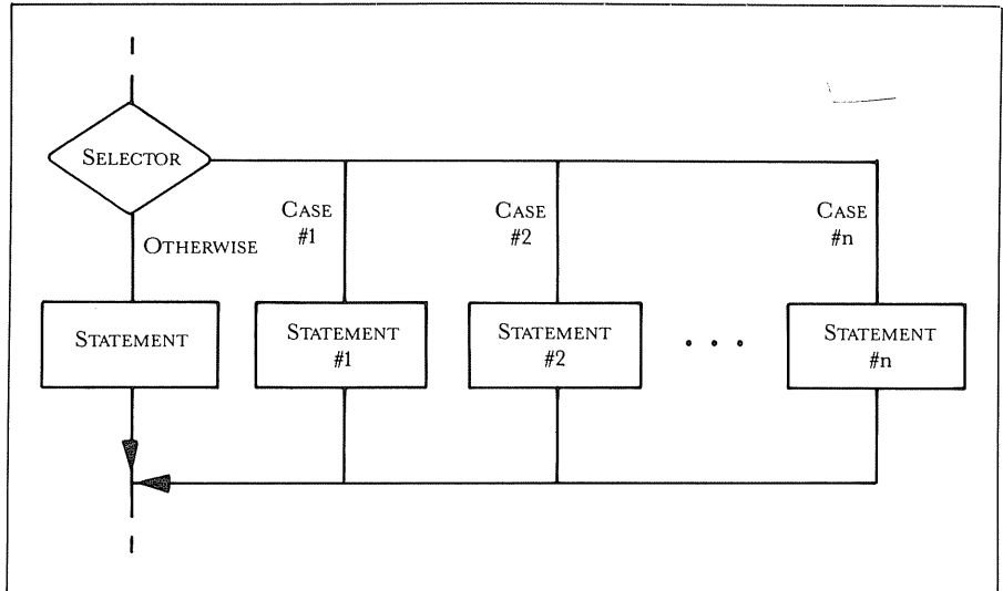
FIGURE 2.4-5: Representing the CASE statement with a flowchart. The form is easily translated into code for languages that do not contain the CASE statement.
