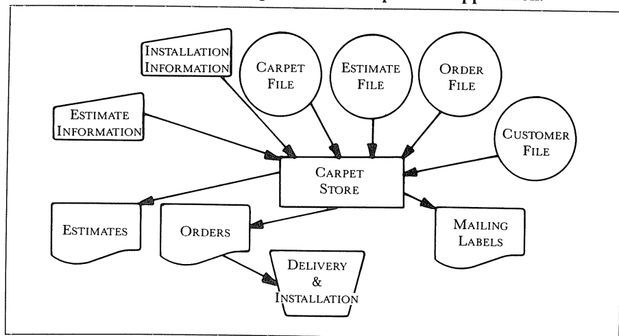
FIGURE 1.4-7: A first attempt at a data flow diagram for the carpet store application.
