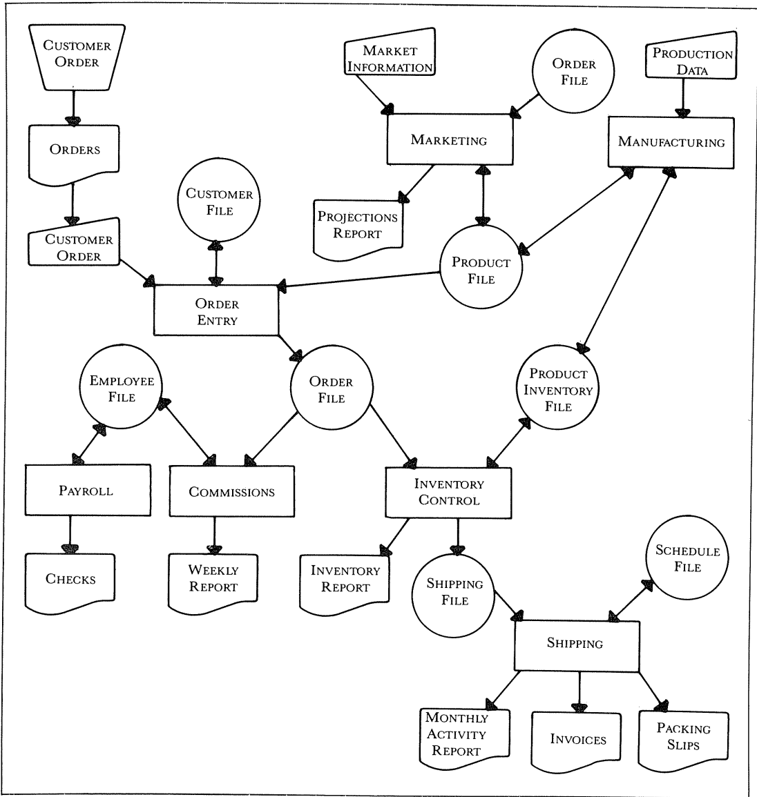
FIGURE 1.4-6: An example of a data flow diagram for a system that might be used by a manufacturing company.
