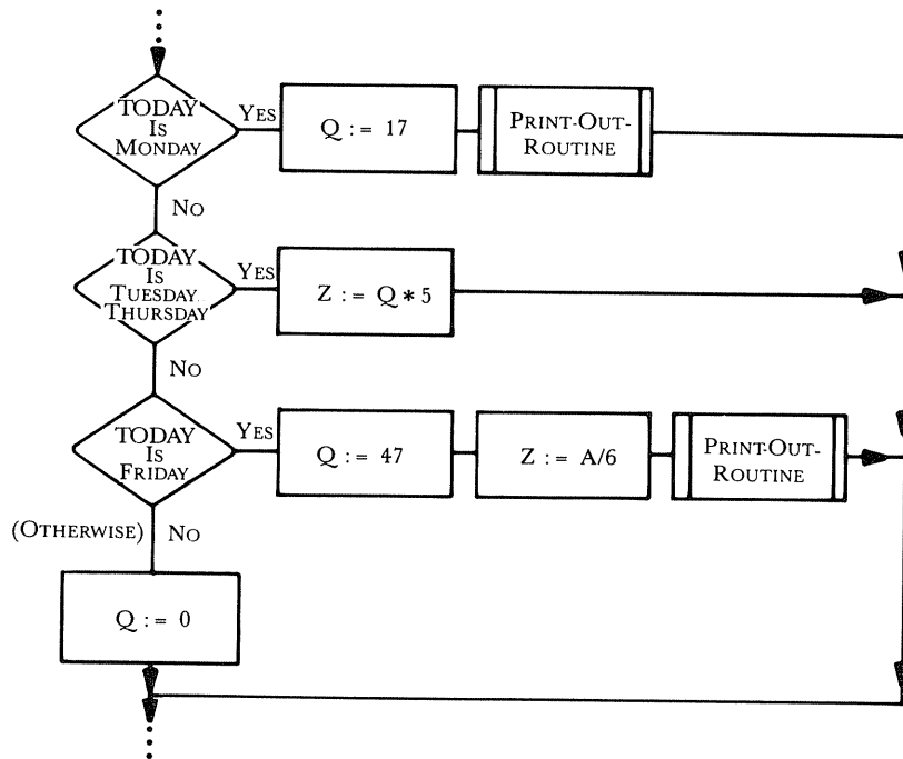
FIGURE 3.2-26a and b: Part (a), top, shows an example of a CASE statement in pseudo-code. There is an obvious problem when trying to translate this statement into a programming language that does not contain a CASE statement. Part (b), bottom, shows how this pseudo-code can be drawn in a flowchart. Part (c), top right, shows how this flowchart can then be used to create appropriate code in BASIC, which typically does not contain a CASE statement.
