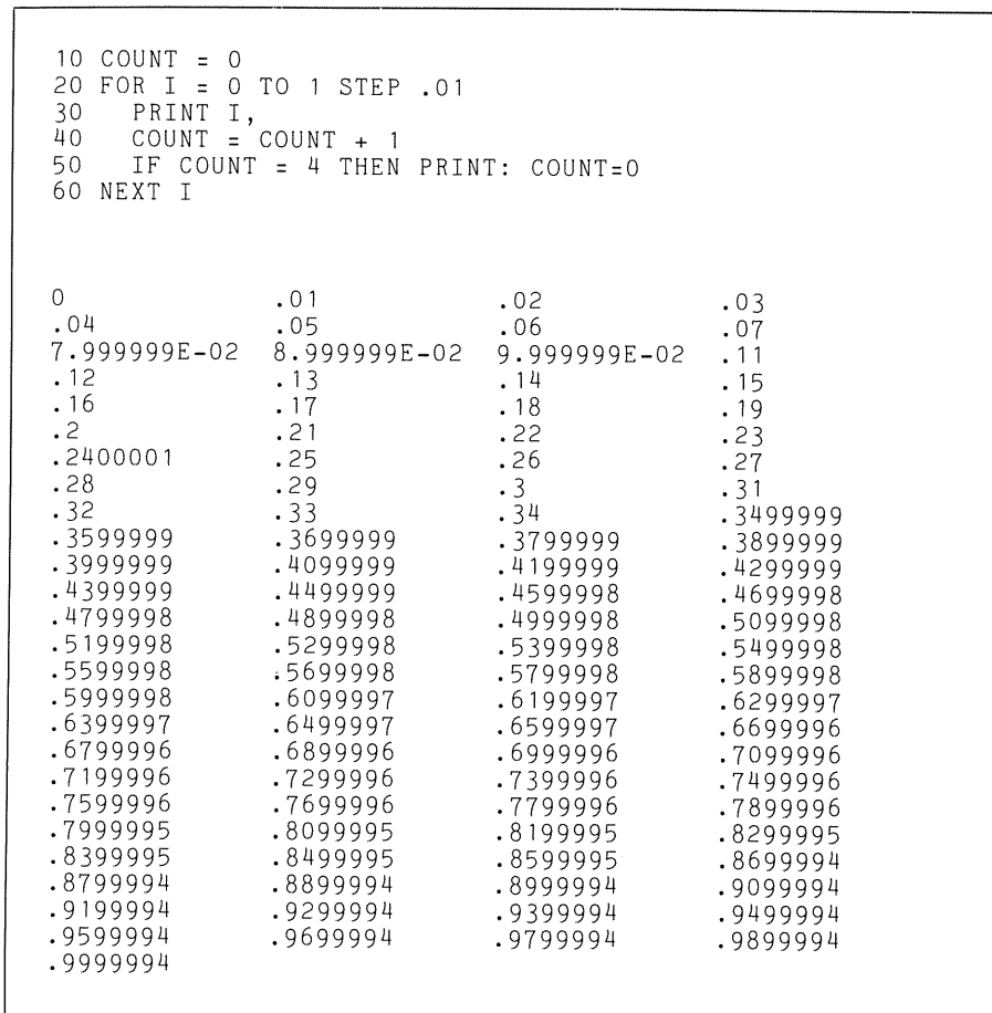
FIGURE 3.2-9: An example of the inaccuracy of floating point numbers.
